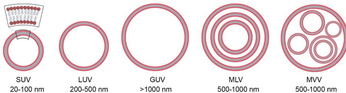
Figure S1. Classification of liposomes according to their size and lamellarity: small unilamellar vesicles (SUV); large unilamellar vesicles (LUV); giant unilamellar vesicles (GUV); multilamellar vesicles (MLV); multivesicular vesicles (MVV).
